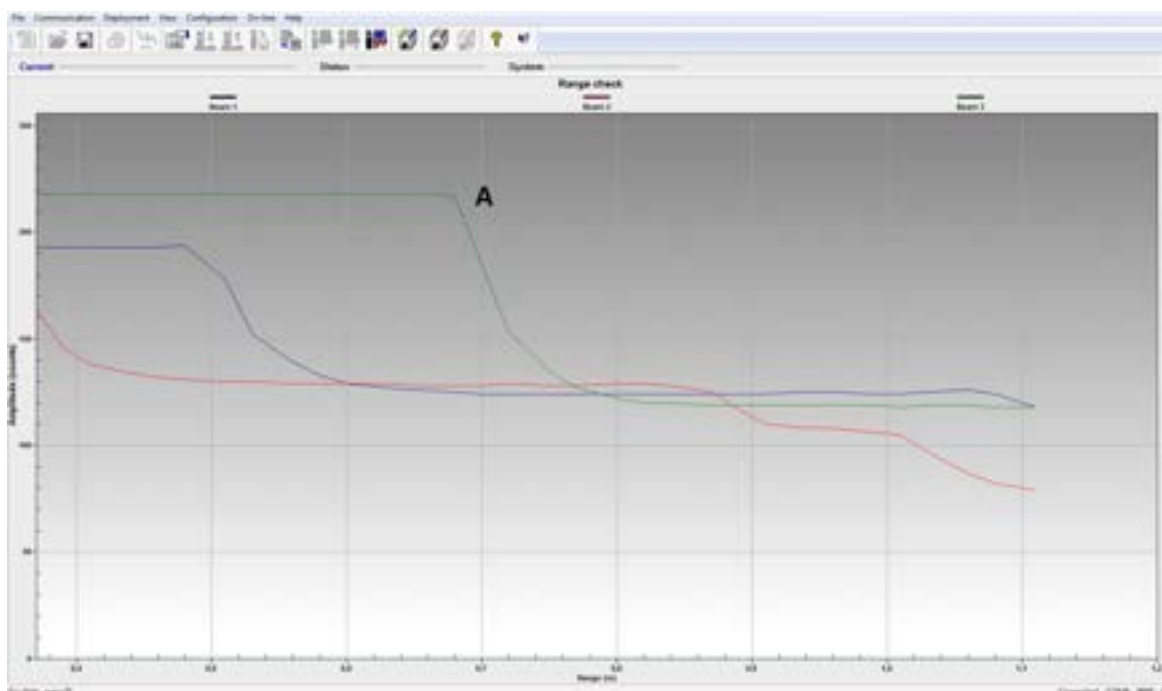
Figure: The kink in the amplitude graph of Beam 3 (A) tells us that the flume wall is 0.7 m away from the transducer.
