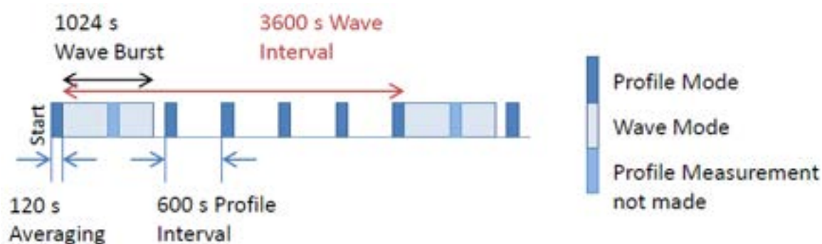
Figure: The AWAC and AquaPro measures profile and waves sequentially. In case of conflict, wave measurements are given priority over profile measurements. Note that the intervals are user selectable in the software; this is just an example.
