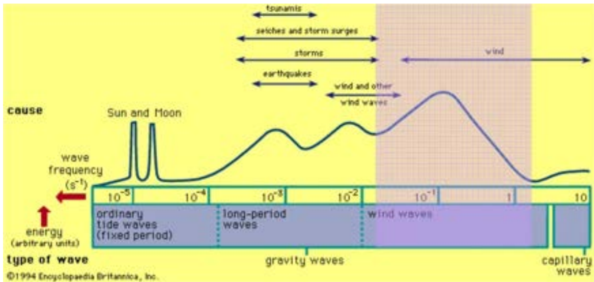
Figure: Distribution of energy. The region with periods from 0.5-30 seconds represents the wind wave band portion of the spectrum. Remember that Period = 1/Frequency.
