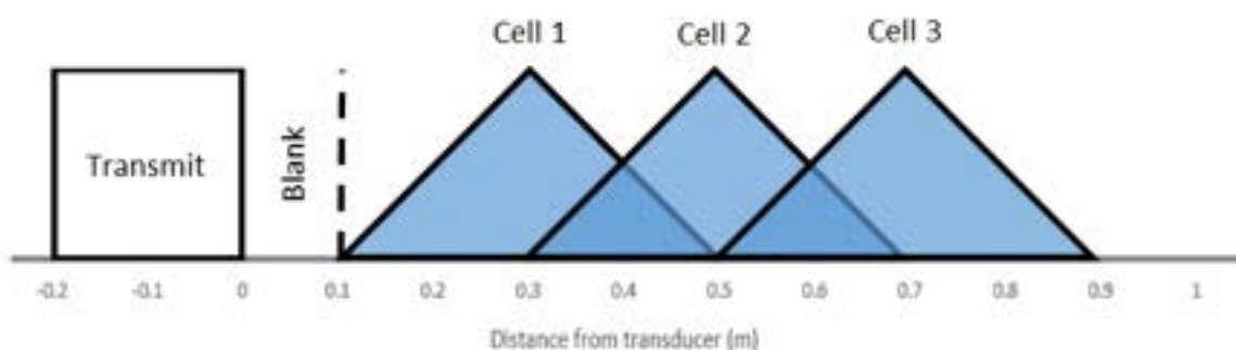
Figure: A series of return signals where the separation between adjacent cells is equal to the length of the transmit pulse. Thi figure shows the triangular weighting given to measurements within each cell, and how these measurement areas overlap due to the transmit pulse length.
