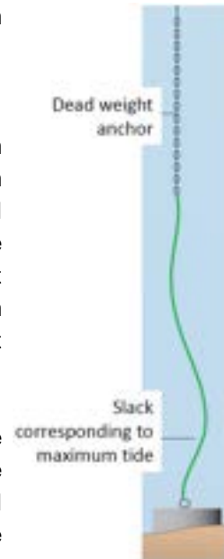
Figure: Illustration of use of dead weight anchor
