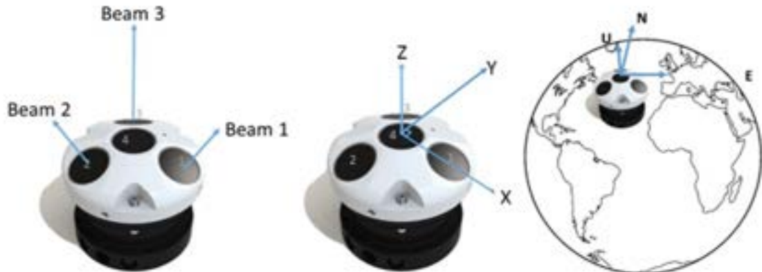
Figure: Coordinate systems. From left: Beam coordinates, XYZ coordinates and ENU coordinates
