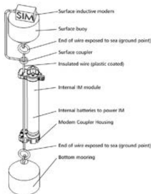
Figure: The main components of an inductive modem system
