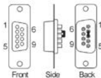
Figure: Serial loop back connector
