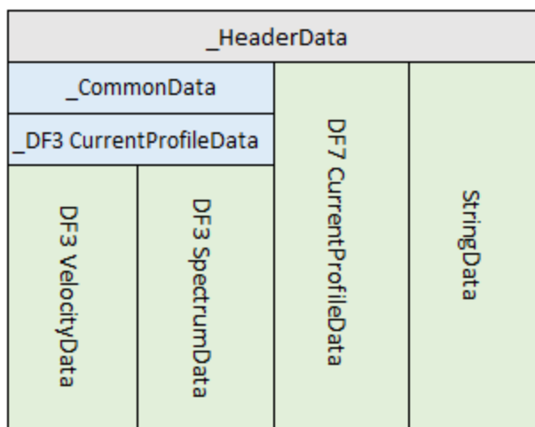
Figure: Showing how common data fields (gray for header and blue for other common's) relate to the sensor specific data fields (green). Note that we use a leading underscore ( ) to emphasize that this is not a sensor data format but is common and used by two or more data formats.
