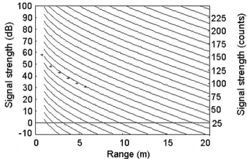
Figure: Measurement range vs signal strength at 2 MHz.
