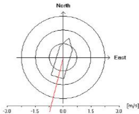
Figure: example of a "raw" current display, i.e. when the heading offset includes correction only for installation offsets, but not compass offsets.
