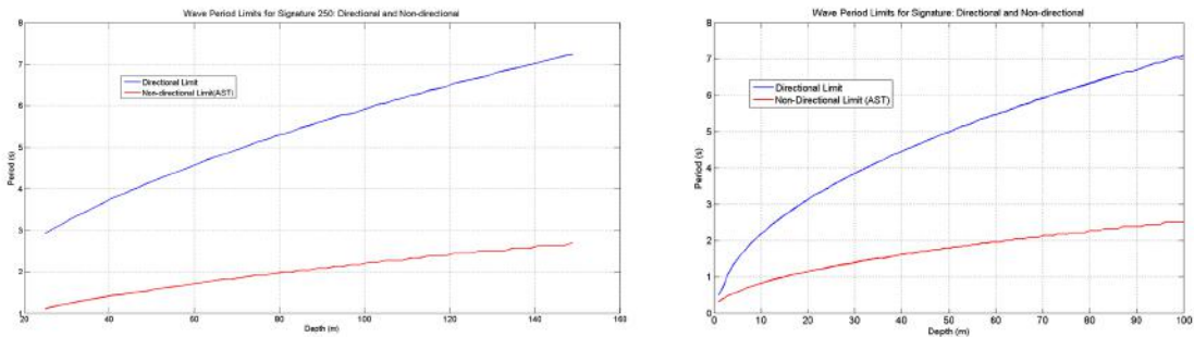
Figure 2: Shows the directional and non-directional limitations for different instrument depths and different wave periods. To the left: Signature 250. Right: Signature1000 and Signature500
