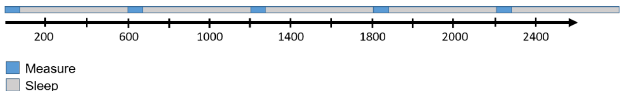
Figure: Sampling sequence when an instrument is configured with a Profiling interval/Measurement interval of 600 sec, and an Average interval of 60 sec.
