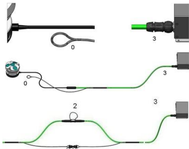
Figure: Nortek Online Cable. Element 0: "Chinese finger trap", 2: Strain relief, 3: Connector to interface box
