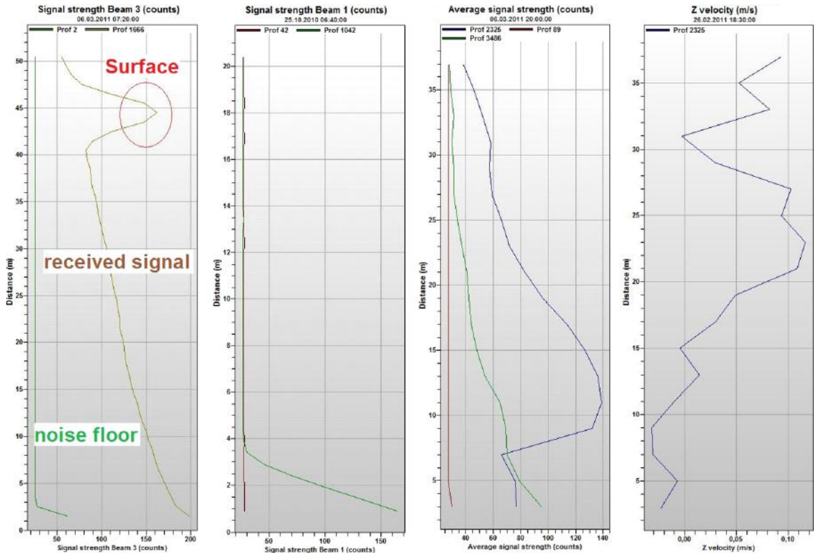
Figure: #1 from left: A good profile. The signal strength profile starts high and exponentially decreases with range. At some point it increase substantially because the transmit pulse has met a boundary (surface or bottom). Note also the Noise Floor profile. The signal should be at least 3 dB higher than the noise floor. #2: Short range. The signal no longer decreases and become constant. It has reached the noise level. No signal is returned to the instrument and the velocity measured is only noise. In this example, the instrument was covered with sand. #3: Blockage. Green profile is a good profile for comparison. Blue profile is increasing at about 10 meters due to blockage. #4: The result of the blockage in Figure #3 is corrupted velocity measurement. This profile shows unreasonable vertical velocity.
