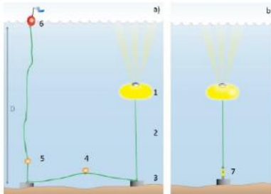
Figure 1: a) is suited for shallow deployments; b) can be used at every depth, provided that the depth capability of the acoustic release (5) or the instrument is not exceeded.
