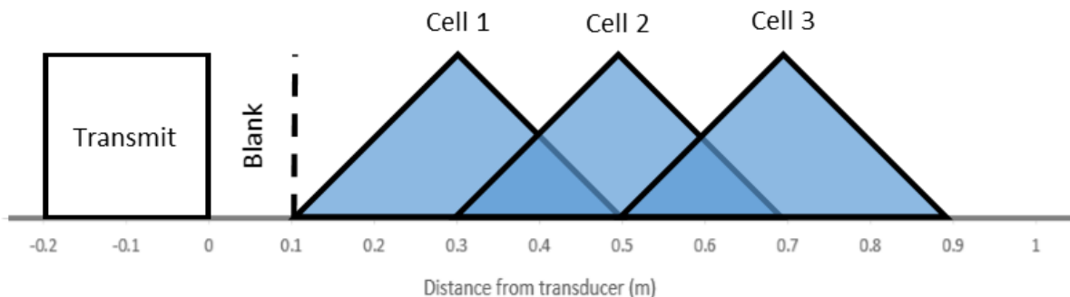
Figure: A series of return signals where the separation between adjacent cells is equal to the length of the transmit pulse. Thi figure shows the triangular weighting given to measurements within each cell, and how these measurement areas overlap due to the transmit pulse length.
