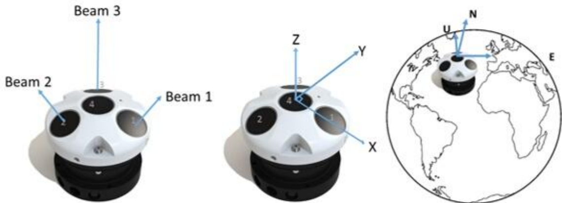
Figure: Coordinate systems. From left: Beam coordinates, XYZ coordinates and ENU coordinates
