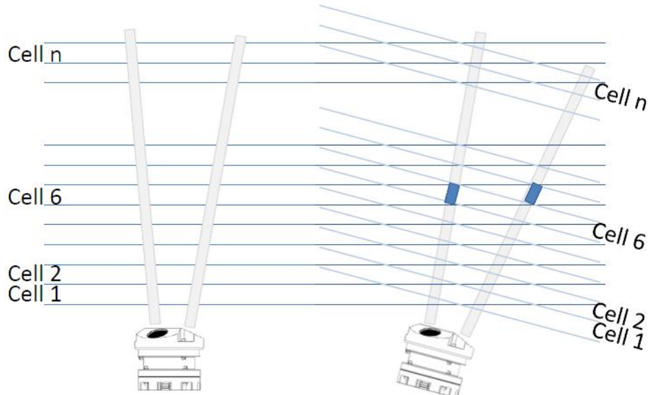
Tilting of the instrument (here 15°) result in measurements from different cells at the same depth.
