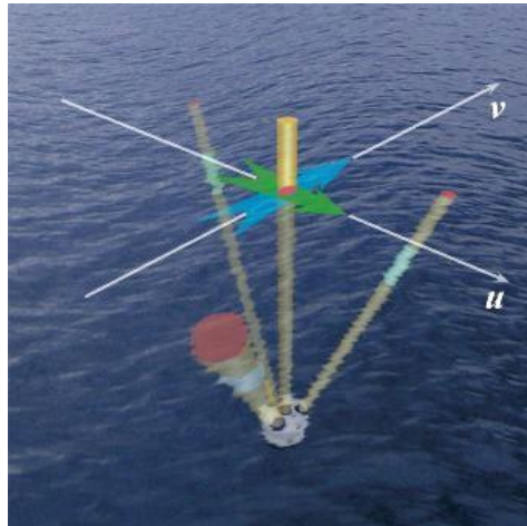
AWAC using the SUV method to capture AST and U/V measurements.
