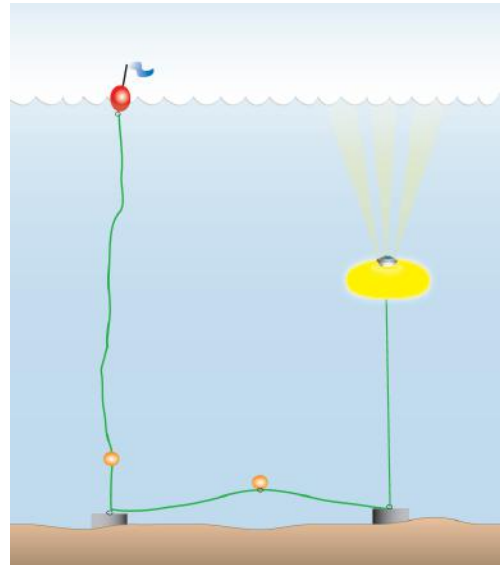
Figure: Subsurface buoy with instrument mounted inside
