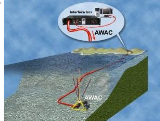
Figure: Bottom mount and online cable
