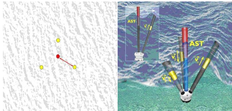
Figure: (a) looking down from above at the array of measurements from the AWAC, and (b) AWAC and the array of measurements cells for orbital velocity measurements (yellow) and the Acoustic Surface Track option (red).
