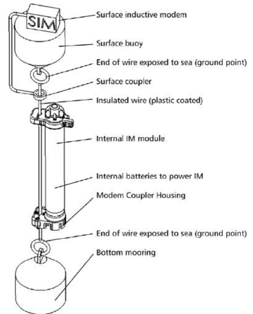
Figure: The main components of an inductive modem system
