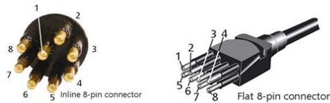
Figure: 8-pin connectors
